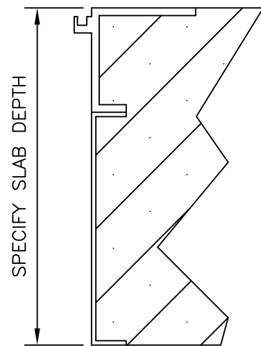
SLAB SKIRTING
