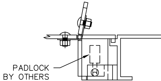
RECESSED LOCK BOX
