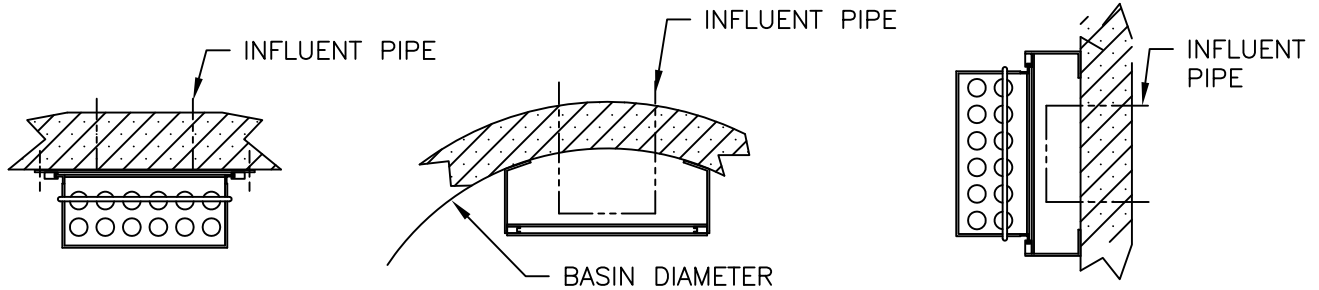
RAILS MOUNTED IN TANK W/FLUSH INFLUENT PIPE
