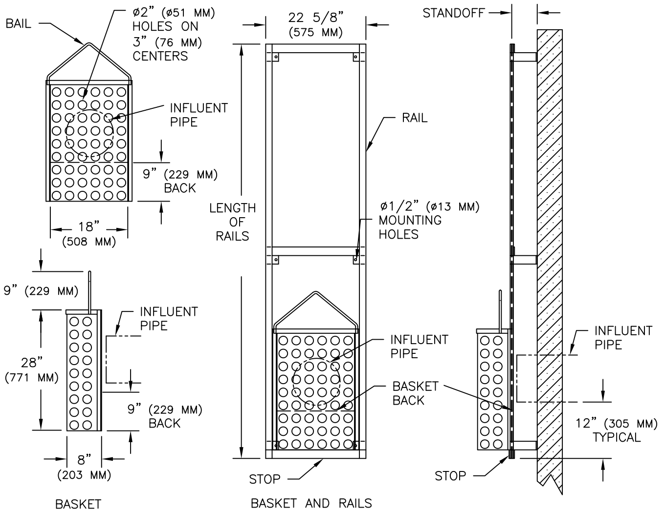
RAILS MOUNTED IN TANK W/FLUSH INFLUENT PIPE
