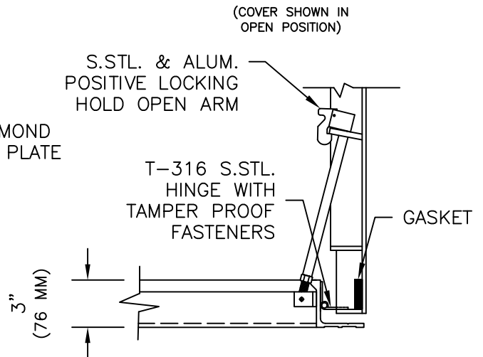
DETAIL
